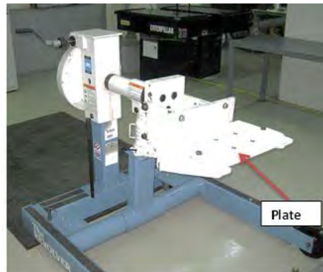
The revolver with the plate for fan group
