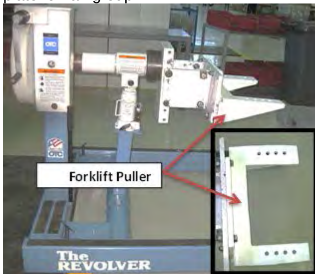
The revolver with the forklift puller for front housings
